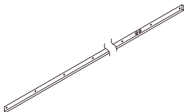
E (x1) Pushrod 5'-7 13/16" x 11/16" x 5/16" (1723*18*8mm)
